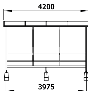
Topaz 207 - 4M
